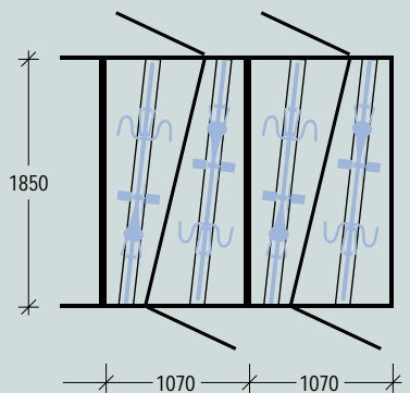
Multiple Unit Configuration Plan View
