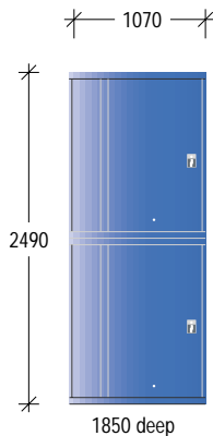
2 Storey Front View
