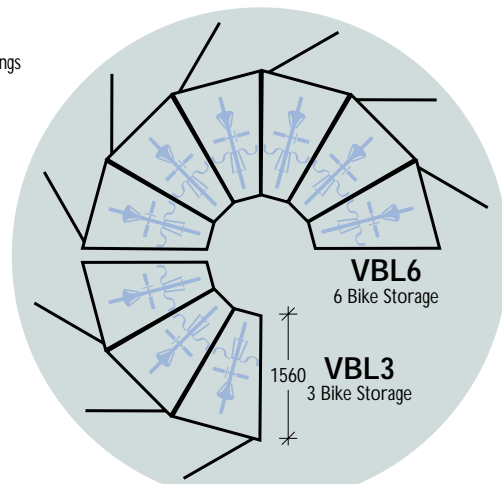
V Shaped Cages Plan Views
