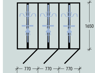
Modular Cages Plan View
